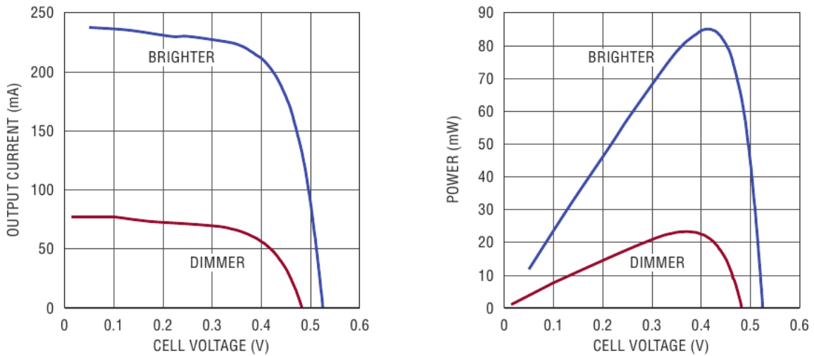
Figure 6: Typical I(V) and power curve of a 2x1 inch ( 13 \text{ cm}^2 ) polycrystalline cell at two different irradiations [1]
